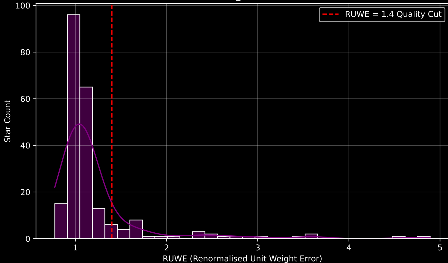
GAPOGEE DR17 Field [232+66_btx] RUWE Distribution (n= 224)
