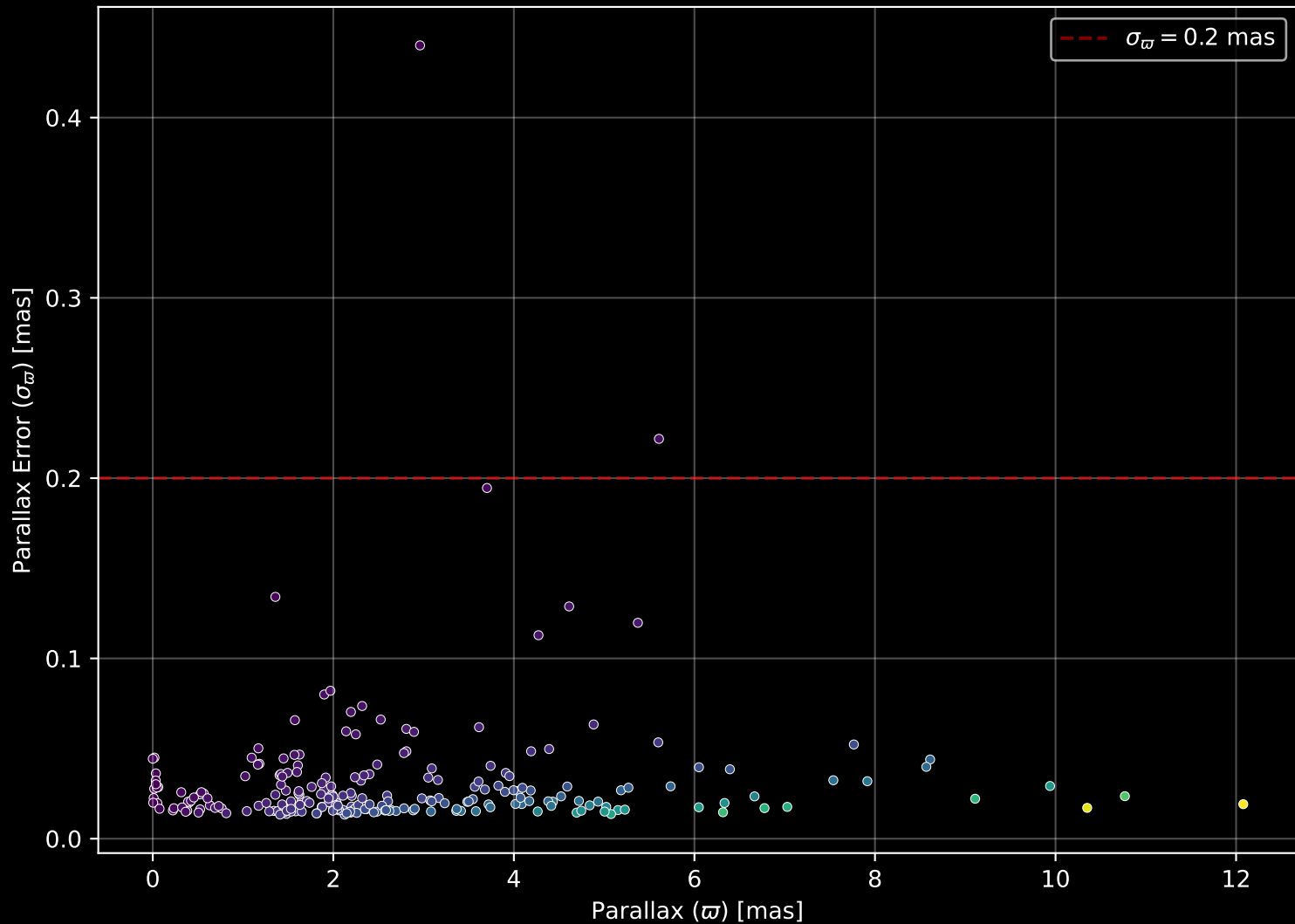
APOGEE DR17 Field: [232+66_btx] Parallax Quality (n= 230)
