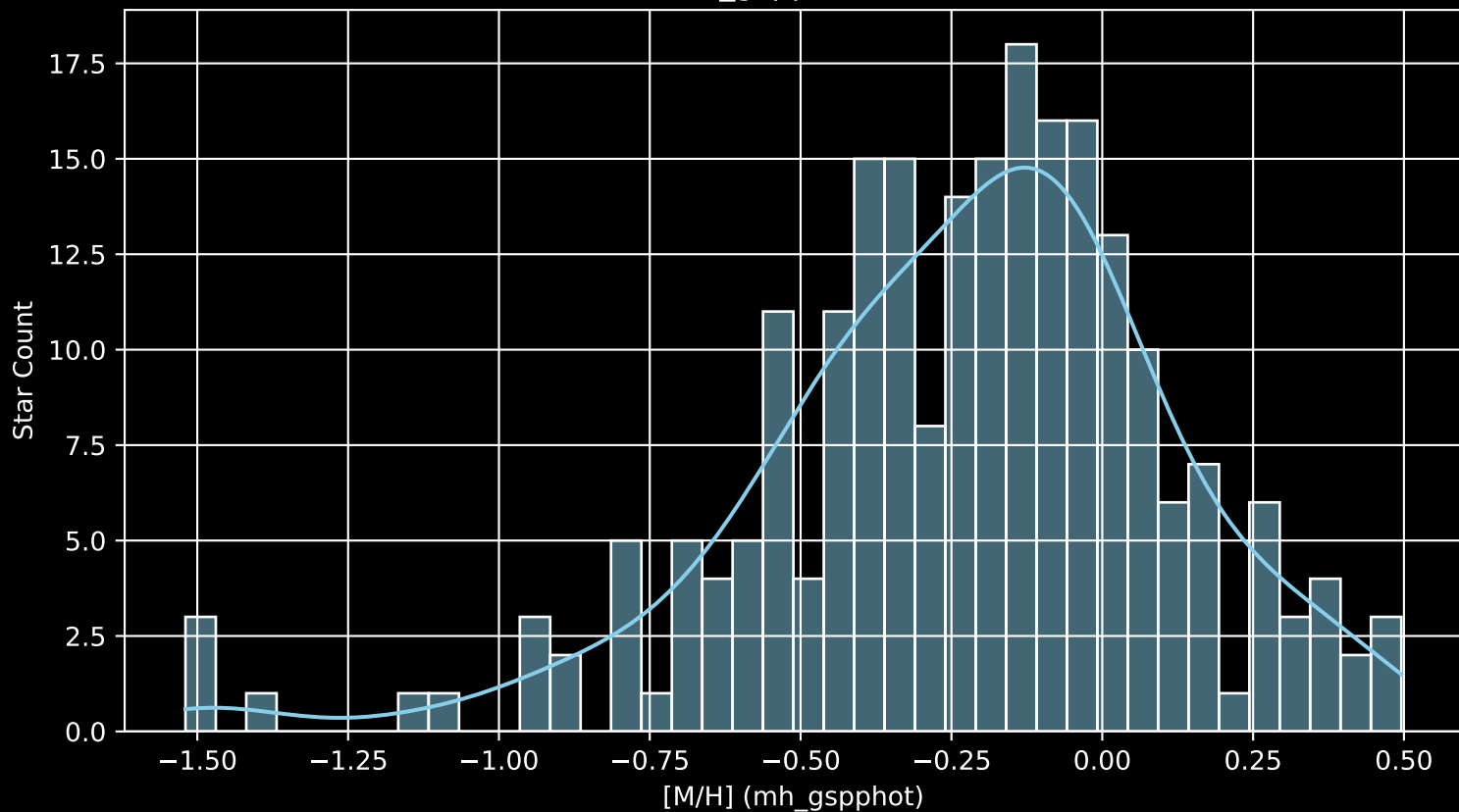
APOGEE DR17 Field: [232+66_btx [M/H] (mh_gspphot) (n= 229)
