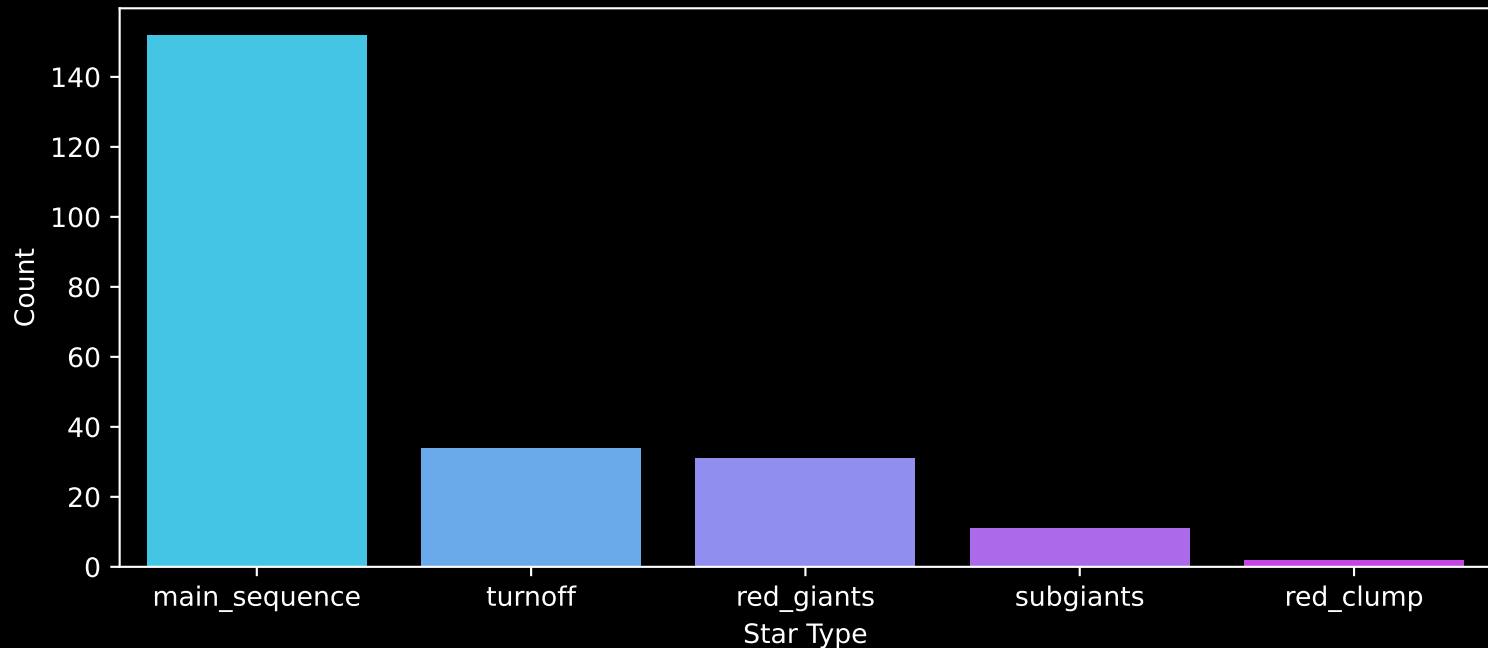
APOGEE DR17 Field: [232+66_btx] Count plot of Star Type
