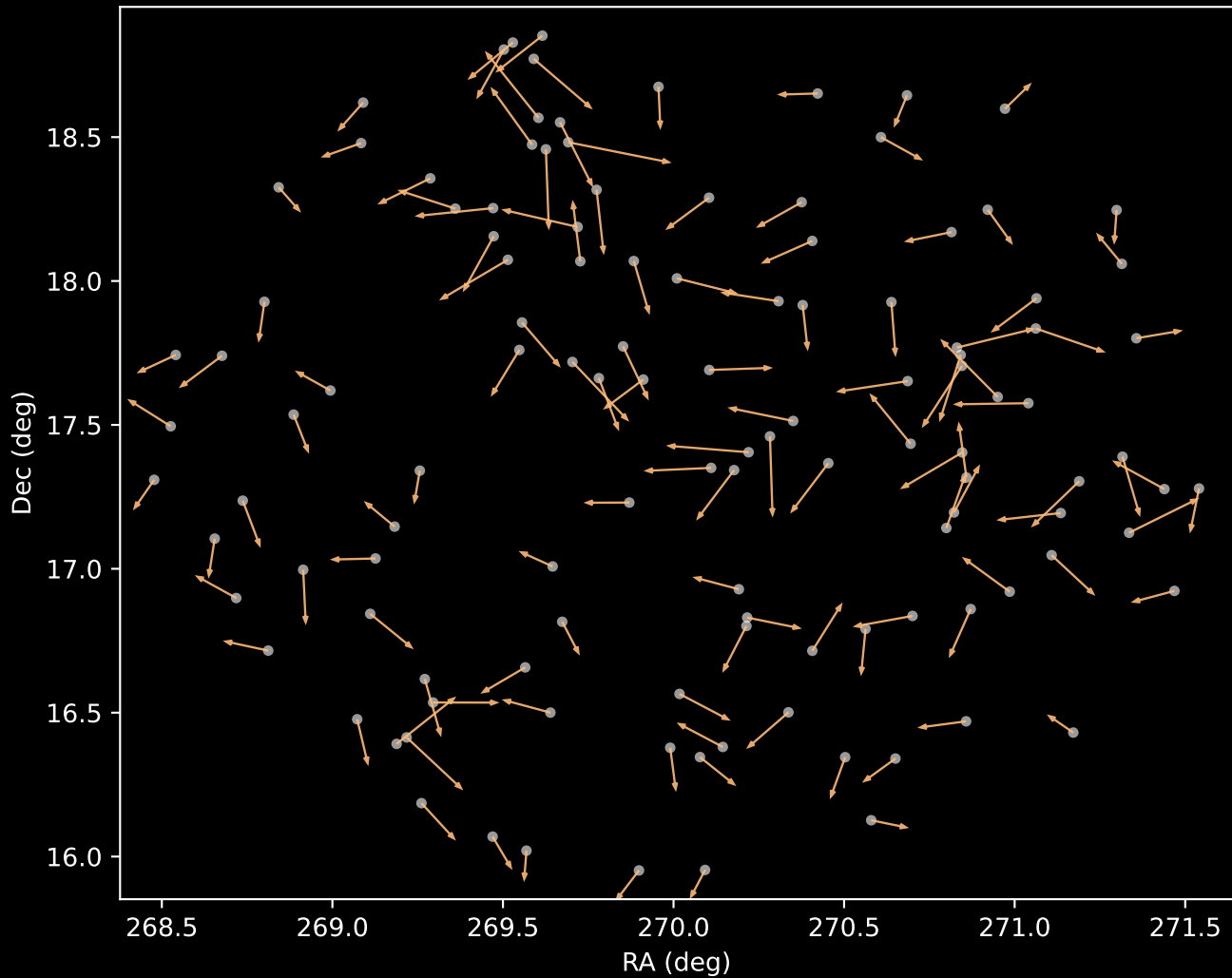
APOGEE DR17 Cluster 3 Proper Motion Vectors (n=121)
