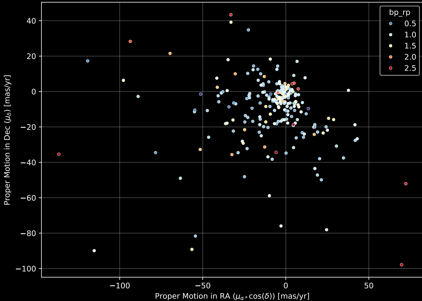
APOGEE DR17 Field: [232+66_btx] Proper Motion Diagram (n= 230)
